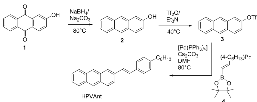
Scheme 1. Synthesis of HPVAnt. Tf = trifluoromethanesulfonyl; DMF = N,N -dimethylformamide.
